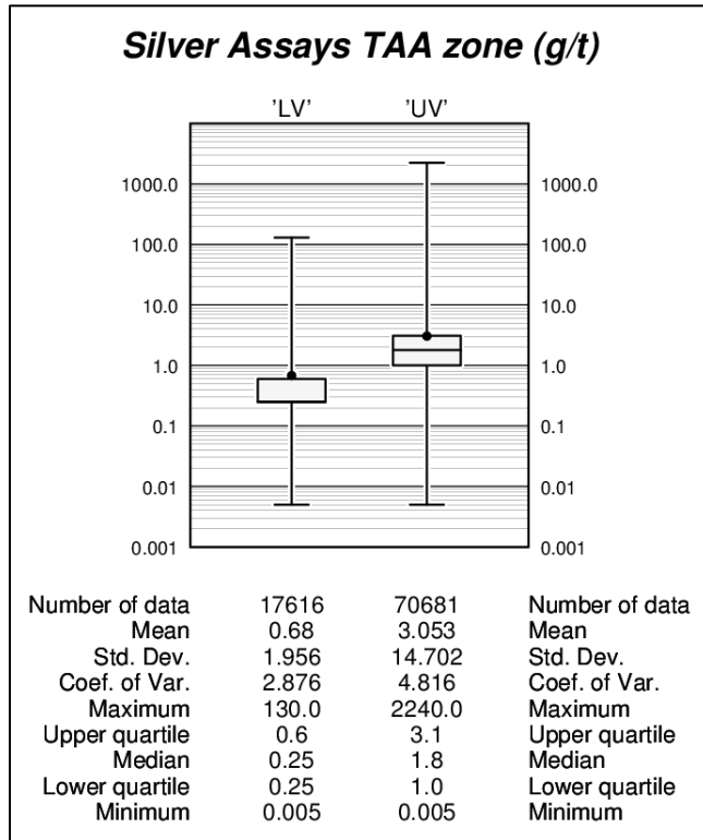
Figure 14-9: Summary Statistics for Silver Assays TAA Zone
