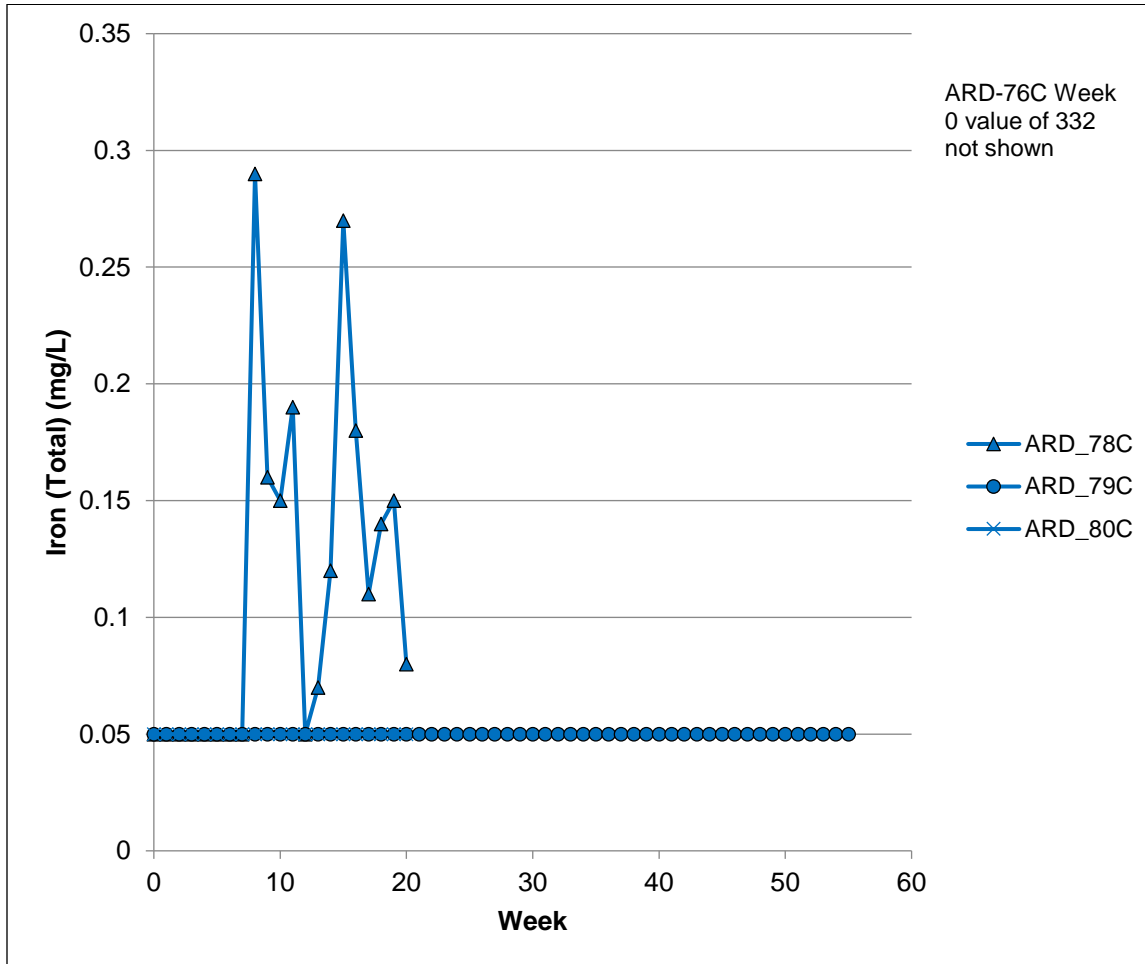
Figure 25-12: Iron Concentration in Leachate from Amulsar Kinetic Cell Results on UV Barren Rock
