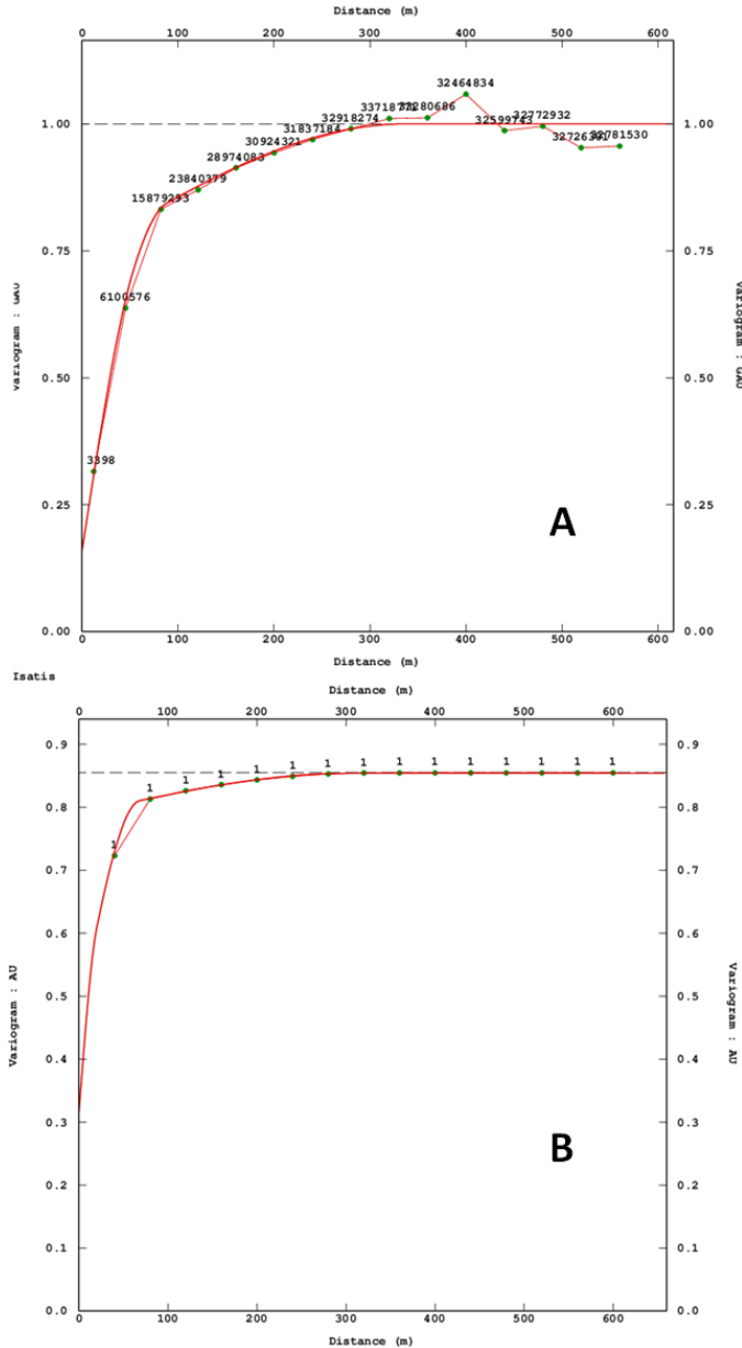
Figure 14-13: Omni-directional Gold Variogram Models TAA UV Domain
