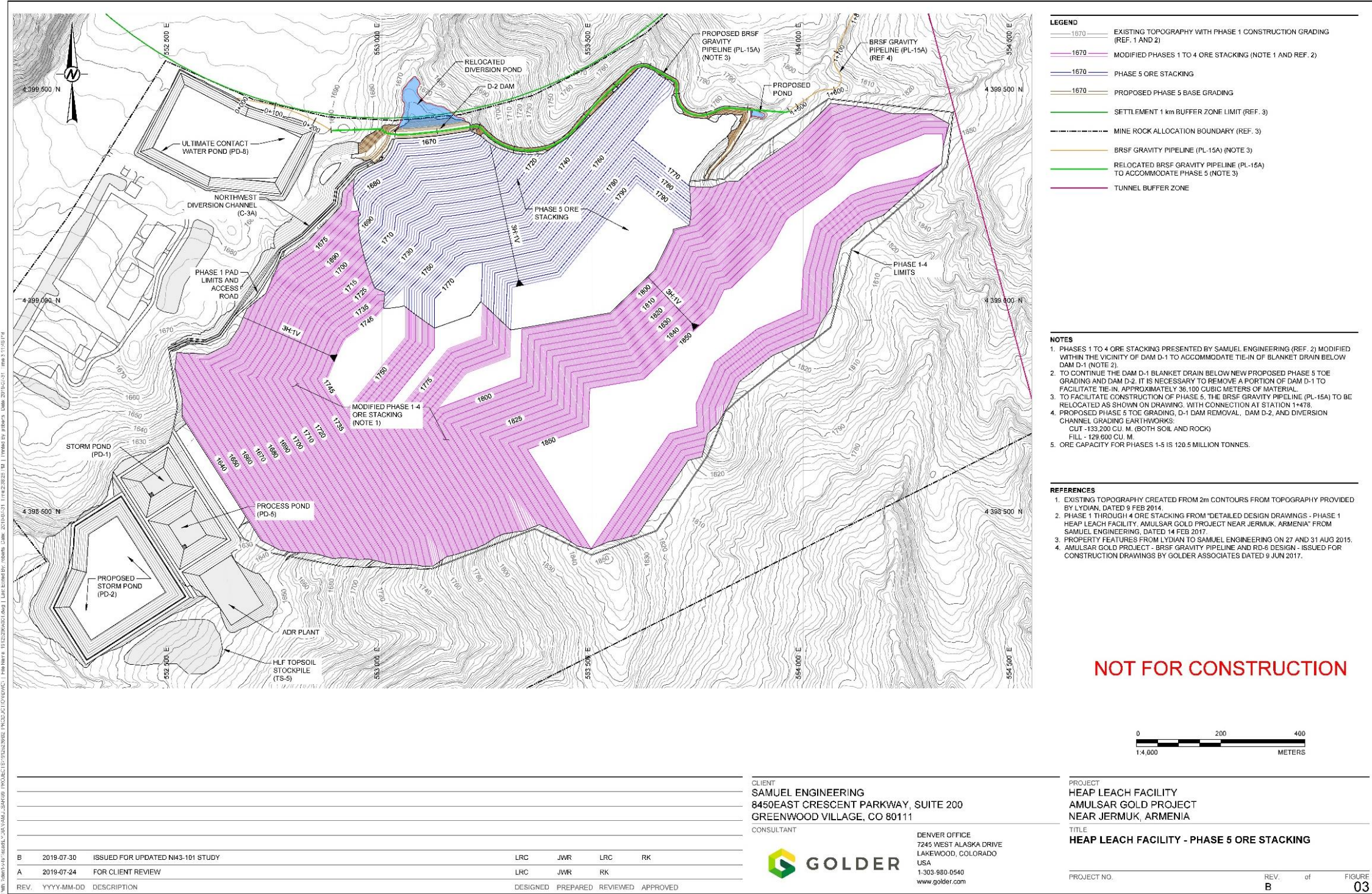
Figure 17-2: Planned Phase 1 to 5 Leach Pad and Ore Heap Plan
